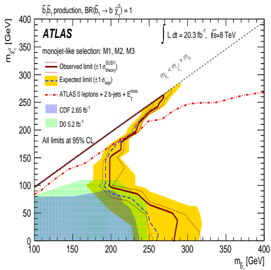
FIG. 11. Exclusion plane at 95% CL as a function of sbottom and neutralino masses for the decay channel \tilde{b}_1 \rightarrow b + \tilde{\chi}_1^0 ( \text{BR}=100\% ). The observed (red line) and expected (blue line) upper limits from this analysis are compared to previous results from CDF [29], D0 [30], and ATLAS [23]. For the latter, the area below the dashed-dotted line is excluded. The dotted lines around the observed limit indicate the range of observed limits corresponding to \pm 1\sigma variations on the NLO SUSY cross-section predictions. The shaded area around the expected limit indicates the expected \pm 1\sigma ranges of limits in the absence of a signal. A band for m_{\tilde{b}_1} - m_{\tilde{\chi}_1^0} - m_b < 2 GeV indicates the region in the phase space for which the sbottom can become long-lived.
