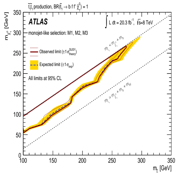
FIG. 10. Exclusion plane at 95% CL as a function of stop and neutralino masses for the decay channel \tilde{t}_1 \rightarrow b + ff' + \tilde{\chi}_1^0 (BR=100%). The dotted lines around the observed limit indicate the range of observed limits corresponding to \pm 1\sigma variations on the NLO SUSY cross-section predictions. The shaded area around the expected limit indicates the expected \pm 1\sigma ranges of limits in the absence of a signal. A band for m_{\tilde{t}_1} - m_{\tilde{\chi}_1^0} - m_b < 2 GeV indicates the region in the phase space for which the stop can become long-lived.
