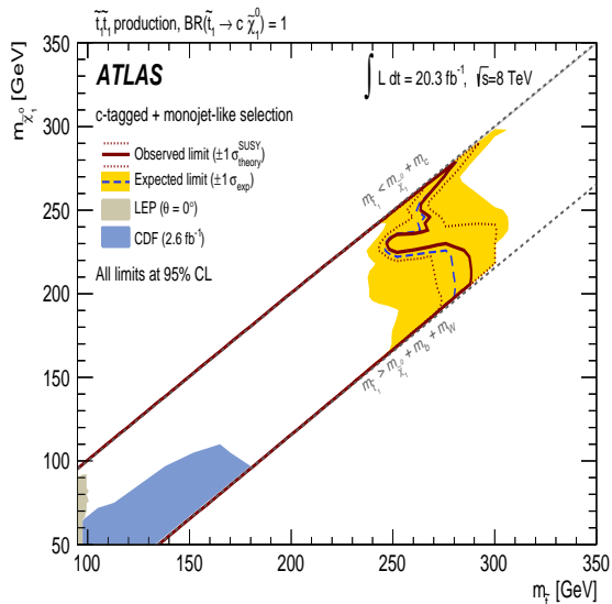
FIG. 9. Exclusion plane at 95% CL as a function of stop and neutralino masses for the decay channel \tilde{t}_1 \rightarrow c + \tilde{\chi}_1^0 (BR=100%). The observed (red line) and expected (blue line) upper limits from this analysis are compared to previous results from Tevatron experiments [27, 28], and from LEP [26] experiments at CERN with squark mixing angle \theta = 0^\circ . The dotted lines around the observed limit indicate the range of observed limits corresponding to \pm 1\sigma variations on the NLO SUSY cross-section predictions. The shaded area around the expected limit indicates the expected \pm 1\sigma ranges of limits in the absence of a signal. A band for \Delta m < 2 GeV indicates the region in the phase space for which the stop can become long-lived.
